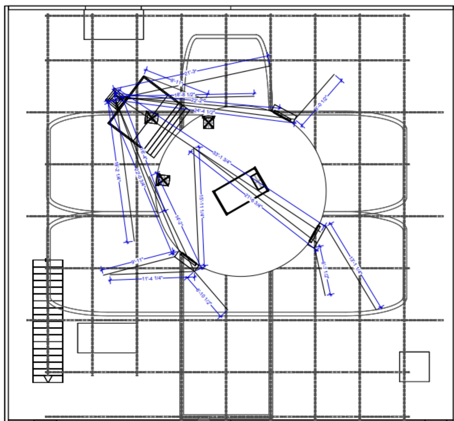
1.5 Wire Ground Plan Scale: 1/4" = 1'-0"
