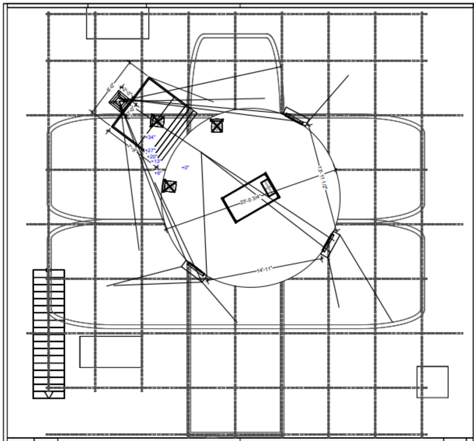
1 Ground Plan Scale: 1/4" = 1'-0"
